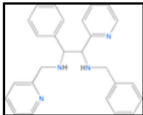
Fig. 1. (1 R *, 2 S *)-N1-benzyl-2-phenyl-1-(pyridin-2-yl)-N2-[(pyridin-2-yl) methyl] ethane-1, 2-diamine
